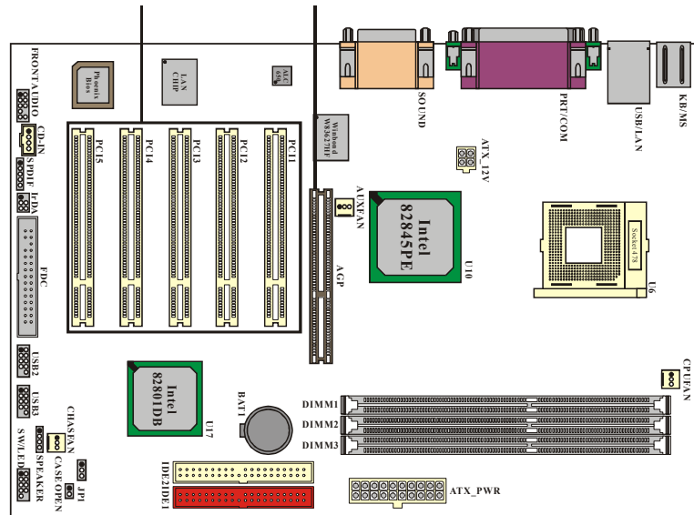
The layout is PX845PEV PRO
