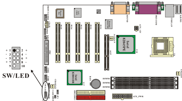
The layout is PX845PEV PRO
