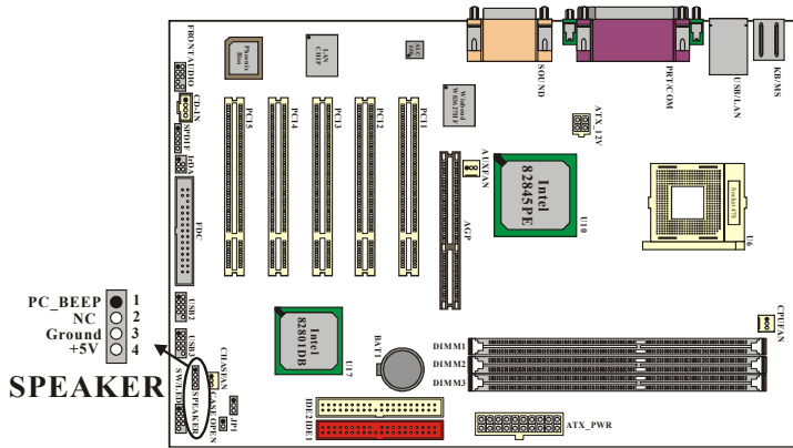
The layout is PX845PEV PRO
