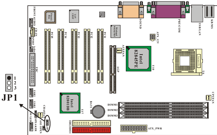
The layout is PX845PEV PRO
