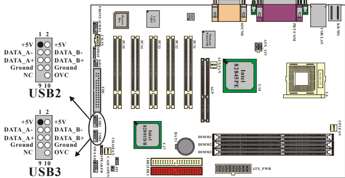
The layout is PX845PEV PRO
